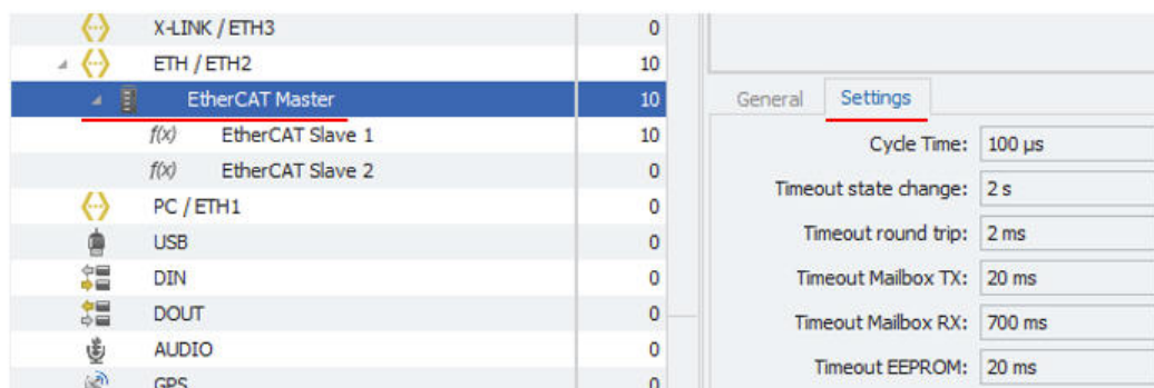
EtherCAT Master settings
