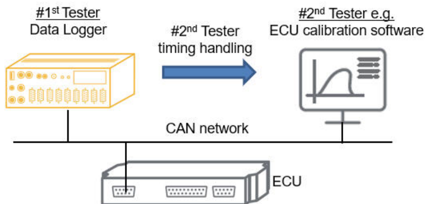
Second tester application
