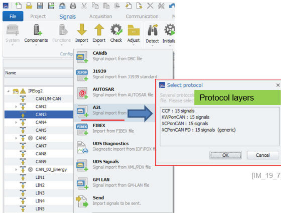
XCP protocol – Select transport layers
