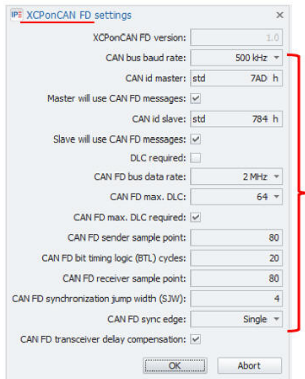
Settings of CAN FD transport layer [IM_19_8]
