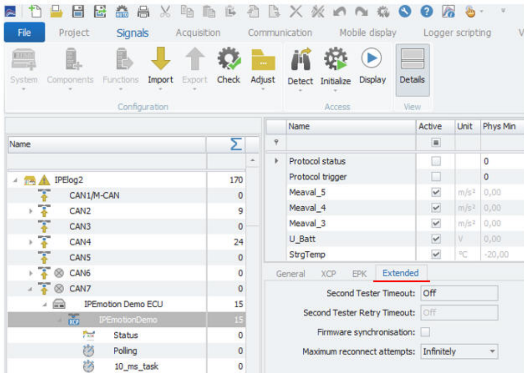
ECU extended second tester settings for CCP and XCP
