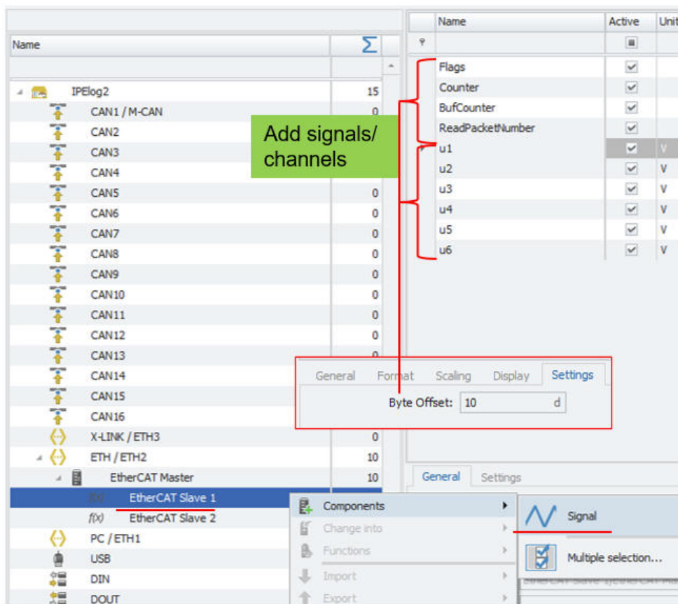
EtherCAT Signal / Channel – define byte offset
