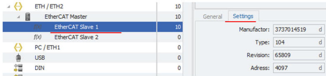
EtherCAT Slave device settings
