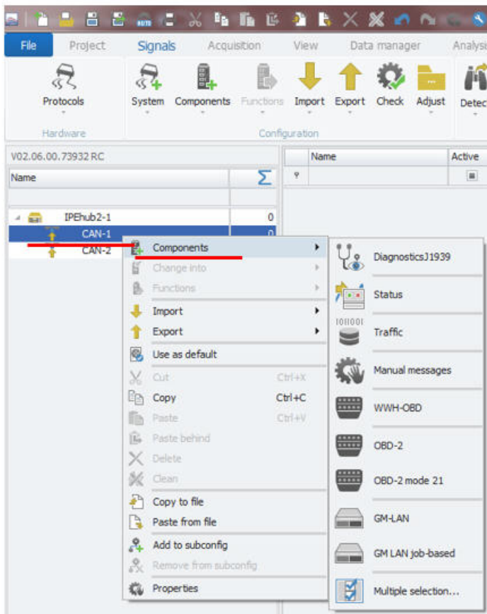
IPEmotion PC: CAN interface components
