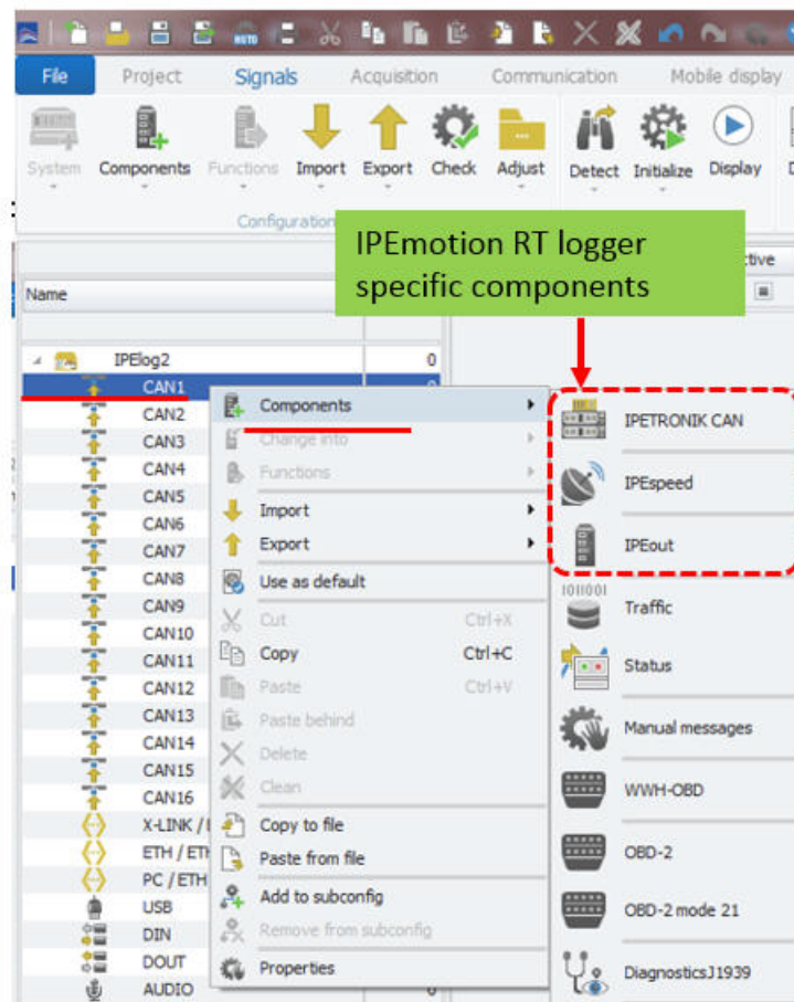
RT Logger: CAN interface components [IM_0_6]
